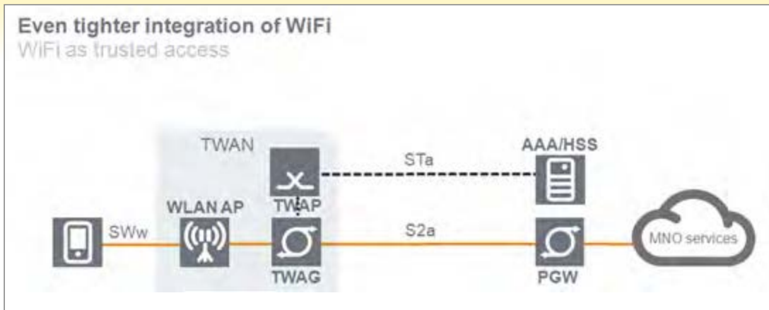
Figure 4: WiFi as trusted access
