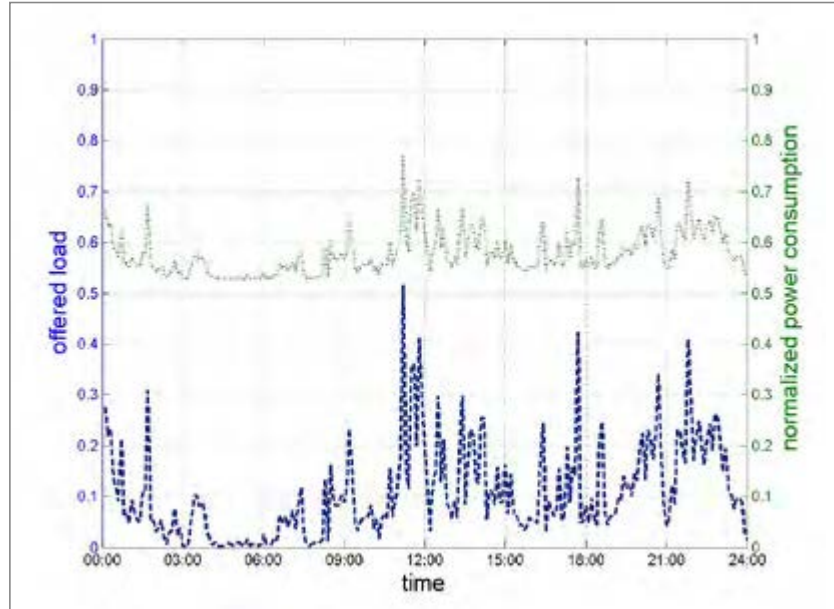
Figure 1: typical traffic evolution and related power consumption of a mobile base station
